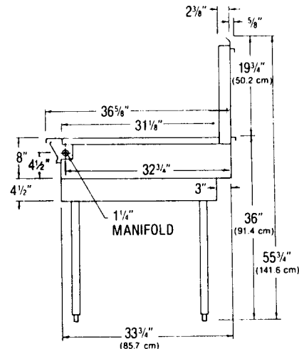
SIDE VIEW MODULAR MODEL WITH HIGH BACK
