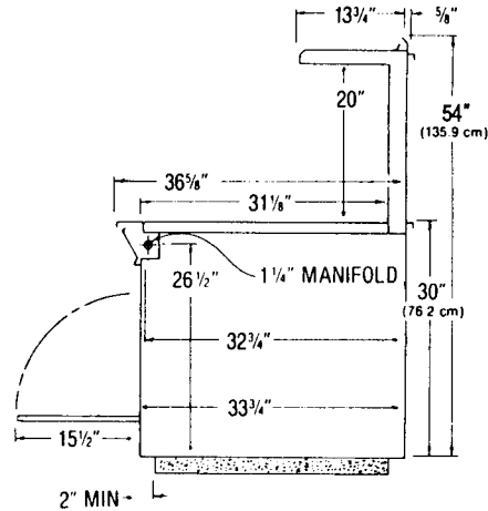
SIDE VIEW WITH SINGLE HIGH SHELF AND CURB MOUNT
